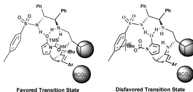
Scheme 2. Proposed transition state in the vinylogous Michael reaction.
